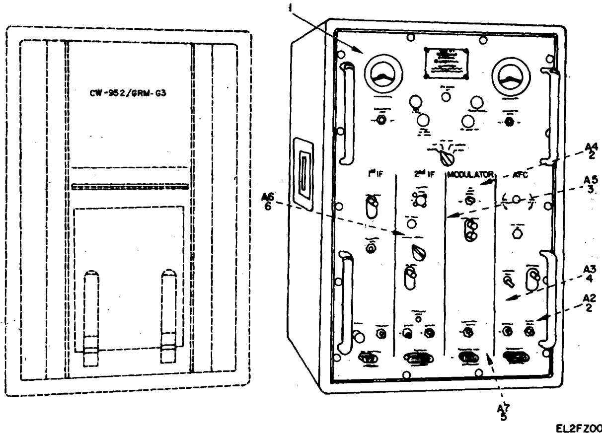
Figure 2. Test Set, Intermediate Frequency TS-2122/GRM-63.
