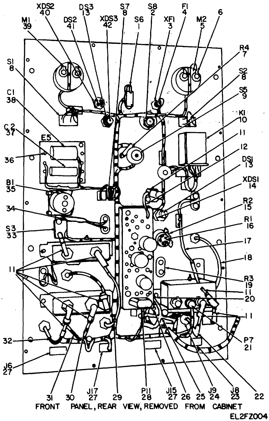
Figure 4. Test Set, Intermediate Frequency TS-2122/GRM-63, Front Panel, Rear View, Removed From Cabinet.
