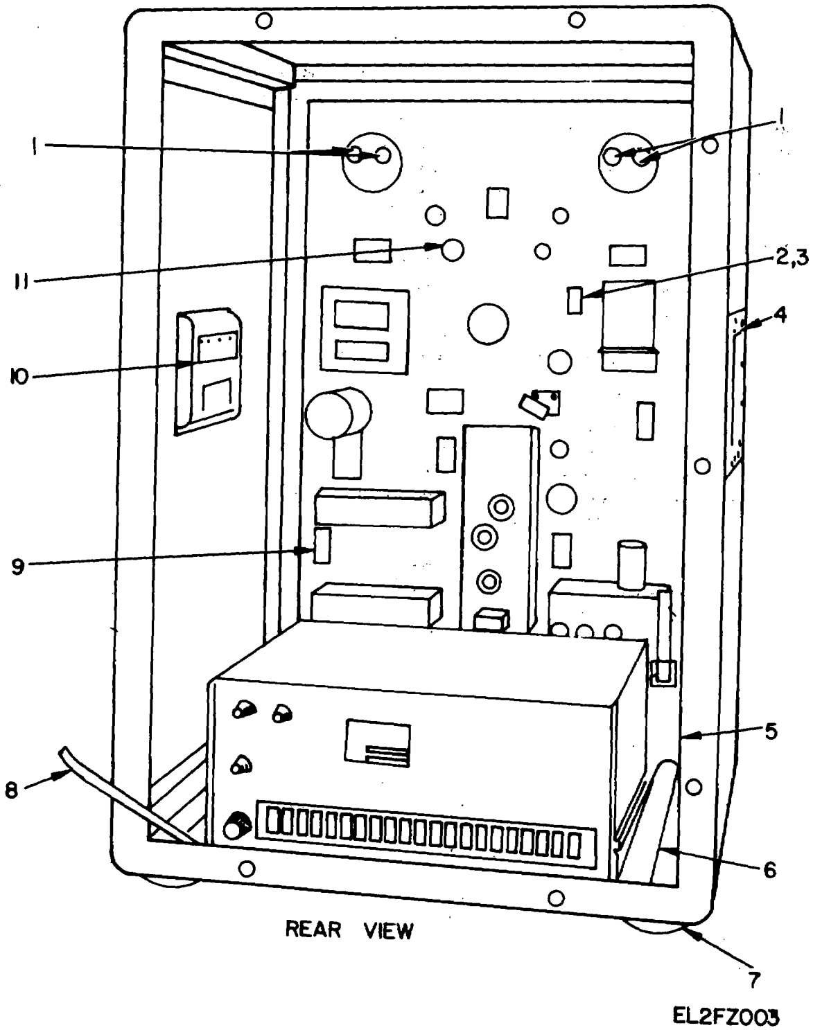
Figure 3. Test Set, Intermediate Frequency TS-2122/GRM-63, Rear View.
