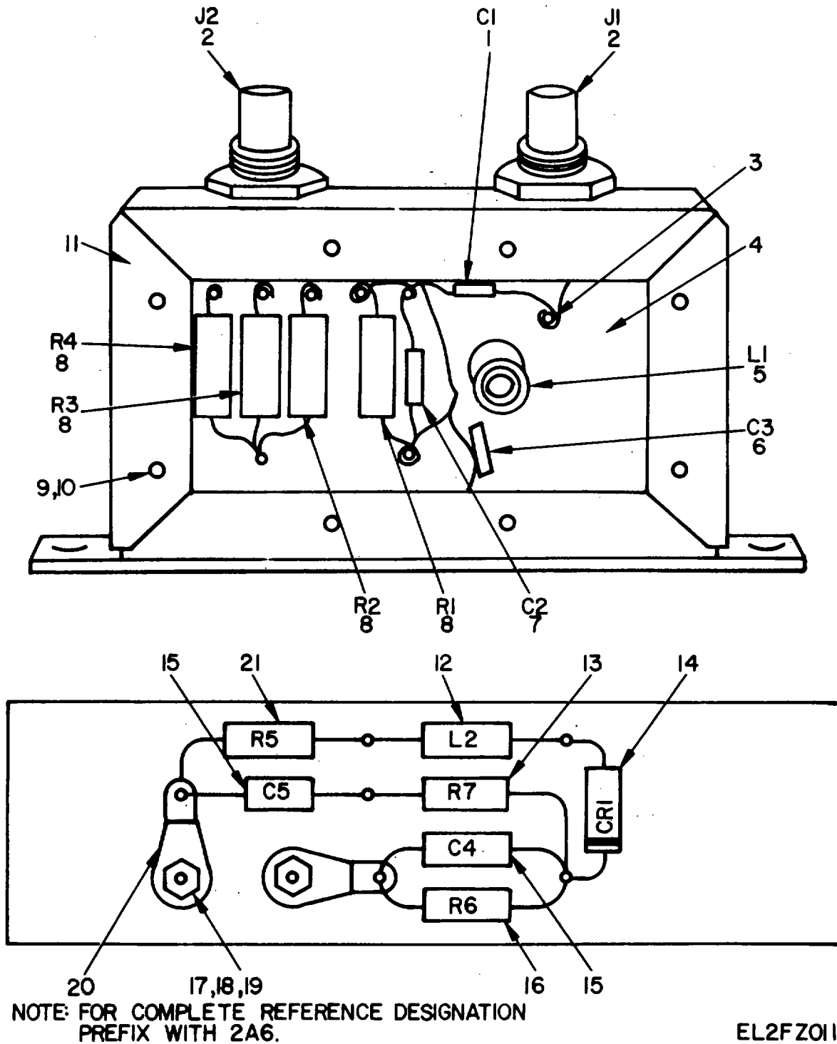
Figure 10. Detector, Modulator Output (2A6).
